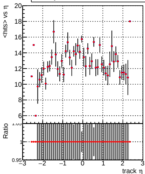
— DQM_V0001_R000000001_Global_CMSSW_NOBATCH_RECO — DQM_V0001_R000000001_Global_CMSSW_BATCH_RECO
