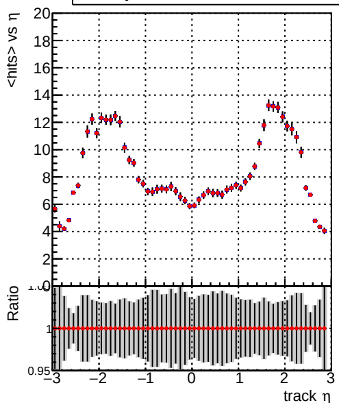
mean hit — DQM_V0001_R000000001_Global_CMSSW_NOBATCH_RECO — DQM_V0001_R000000001_Global_CMSSW_BATCH_RECO
