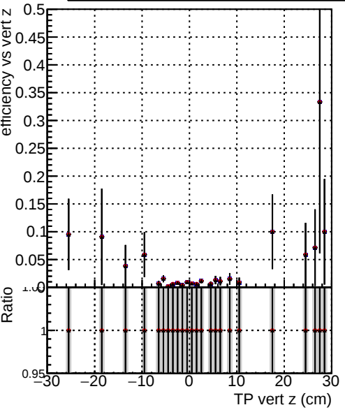
Efficiency vs vertpos —●— DQM_V0001_R000000001_Global_CMSSW_NOBATCH_RECO —●— DQM_V0001_R000000001_Global_CMSSW_BATCH_RECO —●— DQM_V0001_R000000001_Global_CMSSW_FIX_RECO
