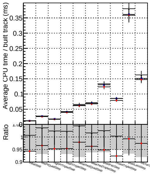
Average CPU time / built track
