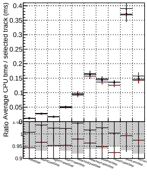
Average CPU time / selected HP track by algoMask
