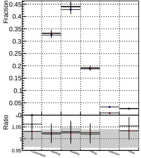
Average Legend: Blue line with dots: DQM_V0001_R000000001_Global_CMSSW_NOBATCH_RECO Red line with dots: DQM_V0001_R000000001_Global_CMSSW_BATCH_RECO Black line with dots: DQM_V0001_R000000001_Global_CMSSW_FIX_RECO
