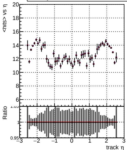
mean hits vs \eta Legend: - DQM_V0001_R0000000001_Global_CMSSW_NOBATCH_RECO (blue line) - DQM_V0001_R0000000001_Global_CMSSW_BATCH_RECO (red line) - DQM_V0001_R0000000001_Global_CMSSW_FIX_RECO (black line)
