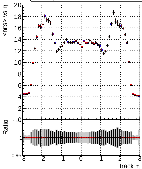
mean hits vs \eta DQM_V0001_R000000001_Global_CMSSW_NOBATCH_RECO DQM_V0001_R000000001_Global_CMSSW_BATCH_RECO DQM_V0001_R000000001_Global_CMSSW_FIX_RECO
