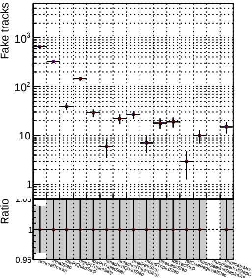
→ DQM_V0001_R0000000001_Global_CMSSW_FIX_RECO
