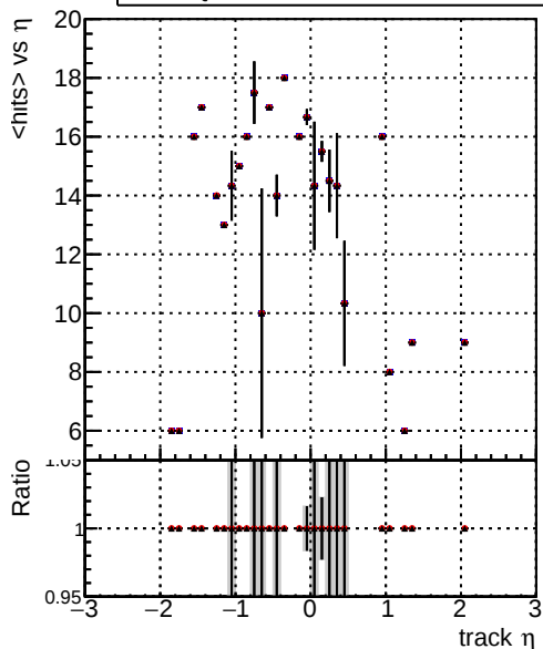
mean hit DQM_V0001_R000000001_Global_CMSSW_NOBATCH_RECO DQM_V0001_R000000001_Global_CMSSW_BATCH_RECO DQM_V0001_R000000001_Global_CMSSW_FIX_RECO
