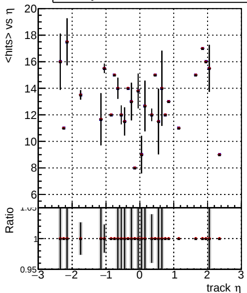
mean hits DQM_V0001_R000000001_Global_CMSSW_NOBATCH_RECO DQM_V0001_R000000001_Global_CMSSW_BATCH_RECO DQM_V0001_R000000001_Global_CMSSW_FIX_RECO
