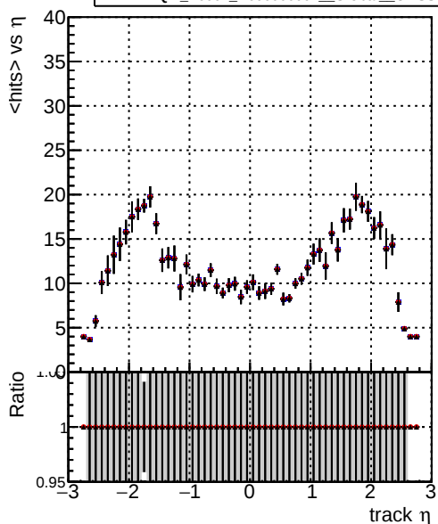
mean hits vs \eta DQM_V0001_R000000001_Global_CMSSW_NOBATCH_RECO DQM_V0001_R000000001_Global_CMSSW_BATCH_RECO DQM_V0001_R000000001_Global_CMSSW_FIX_RECO
