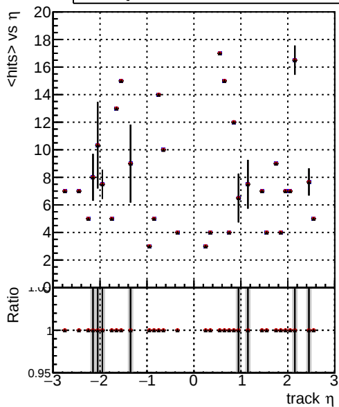
mean hits vs \eta Legend: DQM_V0001_R000000001_Global_CMSSW_NOBATCH_RECO DQM_V0001_R000000001_Global_CMSSW_BATCH_RECO DQM_V0001_R000000001_Global_CMSSW_FIX_RECO
