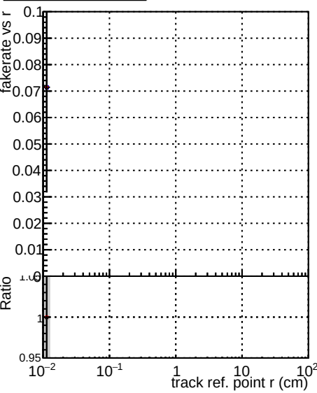
Fake rate vs verpos Global CMSSW NOBATCH RECO Global CMSSW BATCH RECO Global CMSSW FIX RECO
