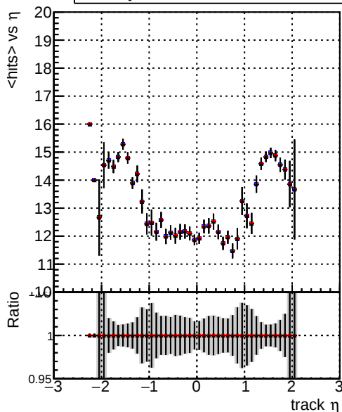
mean hits vs \eta DQM_V0001_R0000000001_Global_CMSSW_NOBATCH_RECO DQM_V0001_R0000000001_Global_CMSSW_BATCH_RECO DQM_V0001_R0000000001_Global_CMSSW_FIX_RECO
