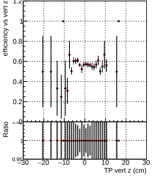
Efficiency vs. TP vert z (cm) —●— DQM_V0001_R0000000001_Global_CMSSW_NOBATCH_RECO —●— DQM_V0001_R0000000001_Global_CMSSW_BATCH_RECO —●— DQM_V0001_R0000000001_Global_CMSSW_FIX_RECO
