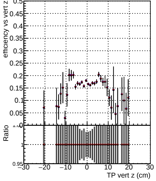
Efficiency vs vert z —●— DQM_V0001_R0000000001_Global_CMSSW_NOBATCH_RECO —●— DQM_V0001_R0000000001_Global_CMSSW_BATCH_RECO —●— DQM_V0001_R0000000001_Global_CMSSW_FIX_RECO
