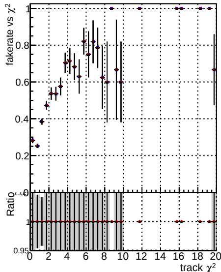
Fake rate vs. Legend Global CMSSW NOBATCH RECO Blue line DOM V0001 DOM V0001 Red line DOM V0001 DOM V0001 Black line DOM V0001 DOM V0001
