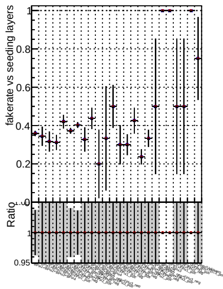
Fake rate vs. Legend Global CMSSW NOBATCH RECO Blue line DOM V0001 DOM V0001 Red line DOM V0001 DOM V0001 Black line DOM V0001 DOM V0001
