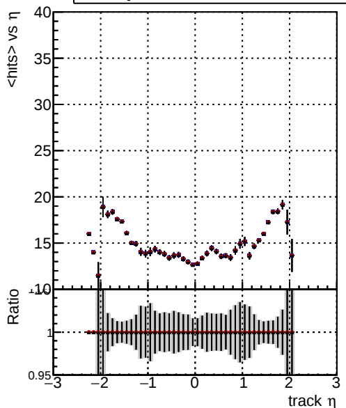
mean hits vs \eta DQM_V0001_R0000000001_Global_CMSSW_NOBATCH_RECO DQM_V0001_R0000000001_Global_CMSSW_BATCH_RECO DQM_V0001_R0000000001_Global_CMSSW_FIX_RECO
