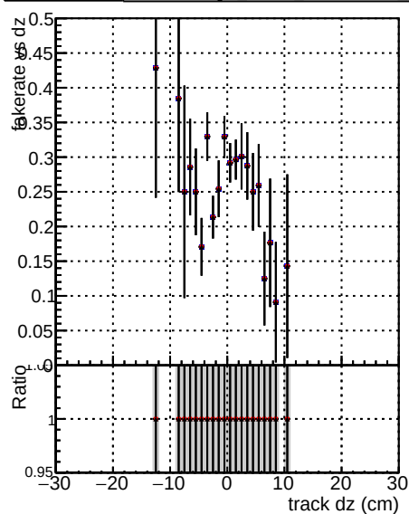
Fake rate vs dz Legend: DOM V0001 R0000000001 Global CMSSW NOBATCH RECO DOM V0001 R0000000001 Global CMSSW BATCH RECO DOM V0001 R0000000001 Global CMSSW FIX RECO
