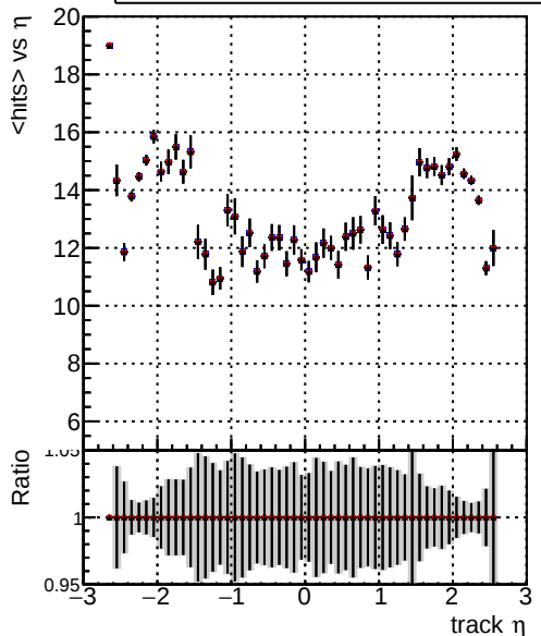
mean hit — DQM_V0001_R000000001_Global_CMSSW_NOBATCH_RECO — DQM_V0001_R000000001_Global_CMSSW_BATCH_RECO — DQM_V0001_R000000001_Global_CMSSW_FIX_RECO
