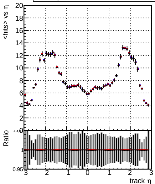
mean hits vs \eta DQM_V0001_R000000001_Global_CMSSW_NOBATCH_RECO DQM_V0001_R000000001_Global_CMSSW_BATCH_RECO DQM_V0001_R000000001_Global_CMSSW_FIX_RECO
