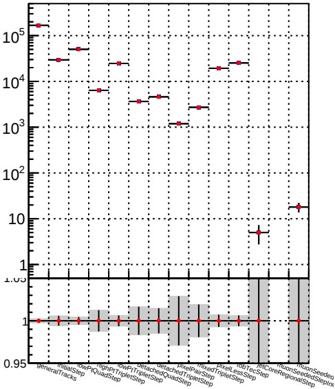
Number —●— DQM_Modified
