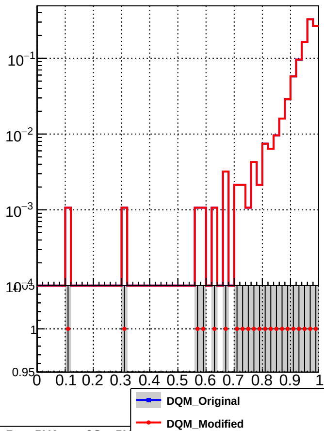
RecoPVAssoc2GenPVMatched_Missing
