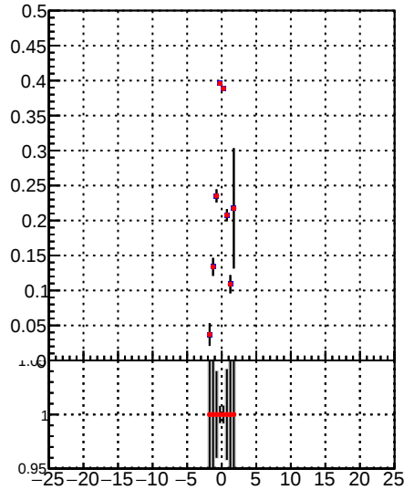
Duplicates Rate vs \Delta y
