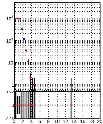
N of reco track vs. \chi^2 — DQM_Original — DQM_Modified
