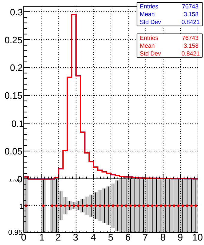
Legend: DQM_Original (grey histogram), DQM_Modified (red line with diamond markers)
