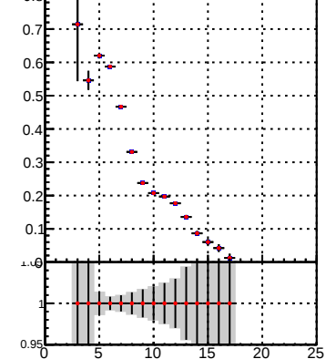
Fake rate vs hit
