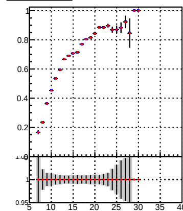
Fake rate vs hit DQM_Original DQM_Modified
