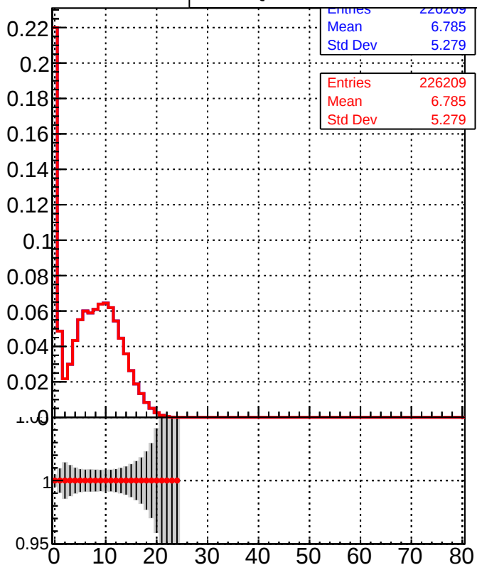
Legend: DQM_Original (grey histogram), DQM_Modified (red line)
