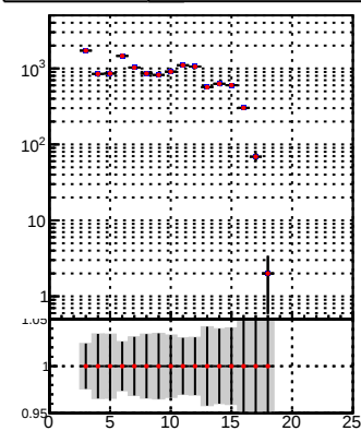
N of reco track vs hit DQM_Original DQM_Modified
