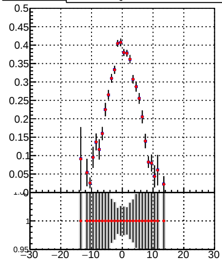
Fake rate vs v Legend: DQM_Original (grey shaded area) DQM_Modified (red line with diamonds)
