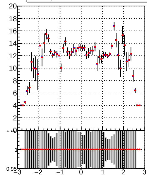
mean hit Legend: DQM_Original (blue line with circles), DQM_Modified (red line with circles)
