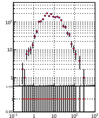
N of reco track vs e DQM_Original DQM_Modified
