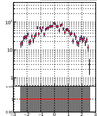
N of reco track vs e DQM_Original DQM_Modified
