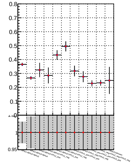
Fake rate vs. —●— DQM Original —●— DQM Modified
