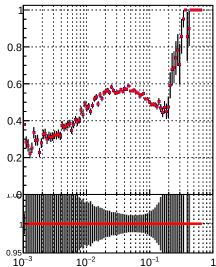
Fake rate vs \sqrt{s} Legend: DQM_Original (blue line), DQM_Modified (red line)
