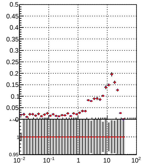
Efficiency vs. \sqrt{s} (GeV) Legend: DQM_Original (blue line with error bars), DQM_Modified (red line with error bars)
