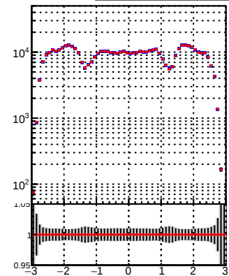
N of reco track vs \eta DQM_Original DQM_Modified
