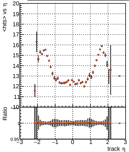
mean hits DQM_V0001_R000000001_Global_CMSSW_orig DQM_V0001_R000000001_Global_CMSSW_pl08 DQM_V0001_R000000001_Global_CMSSW_pl075 DQM_V0001_R000000001_Global_CMSSW_pl07
