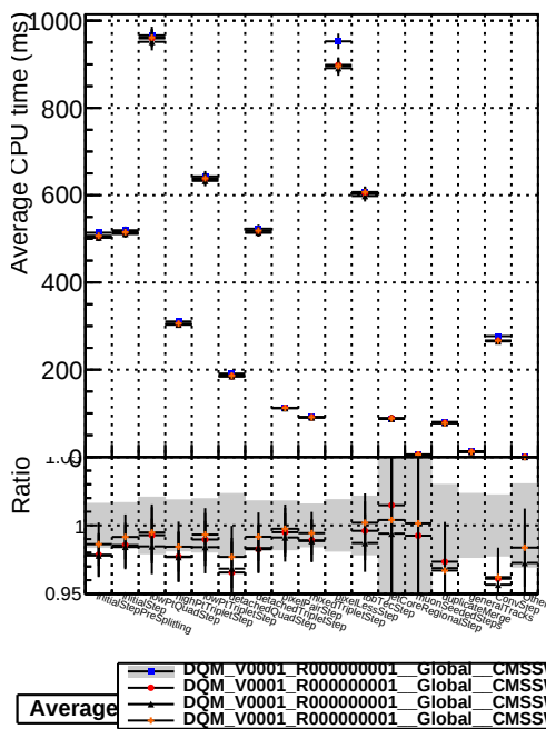
Average CPU time / event
