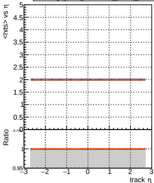
mean hit DQM_V0001_R000000001 Global CMSSW_018 DQM_V0001_R000000001 Global CMSSW_075 DQM_V0001_R000000001 Global CMSSW_017
