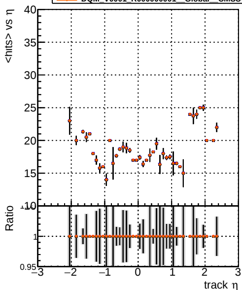
mean hits vs \eta DQM_V0001_R000000001 Global CMSSW_orig DQM_V0001_R000000001 Global CMSSW_pl08 DQM_V0001_R000000001 Global CMSSW_pl075 DQM_V0001_R000000001 Global CMSSW_pl07
