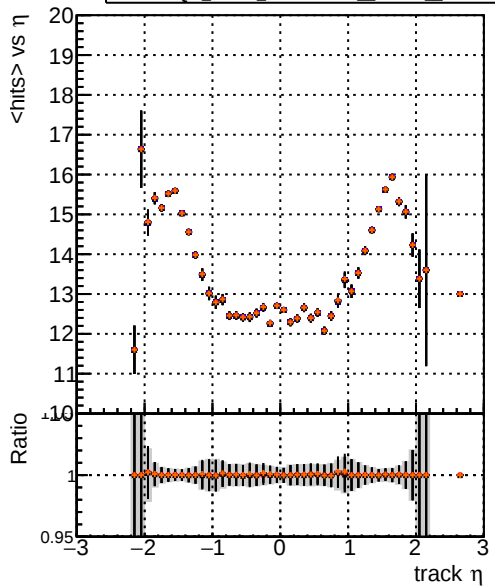
mean hit DQM_V0001_R000000001 Global CMSSW_orig DQM_V0001_R000000001 Global CMSSW_pl08 DQM_V0001_R000000001 Global CMSSW_pl075 DQM_V0001_R000000001 Global CMSSW_pl07
