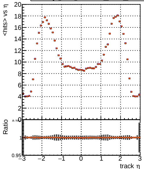
mean hit DQM_V0001_R000000001_Global_CMSSW_orig DQM_V0001_R000000001_Global_CMSSW_pl08 DQM_V0001_R000000001_Global_CMSSW_pl075 DQM_V0001_R000000001_Global_CMSSW_pl07
