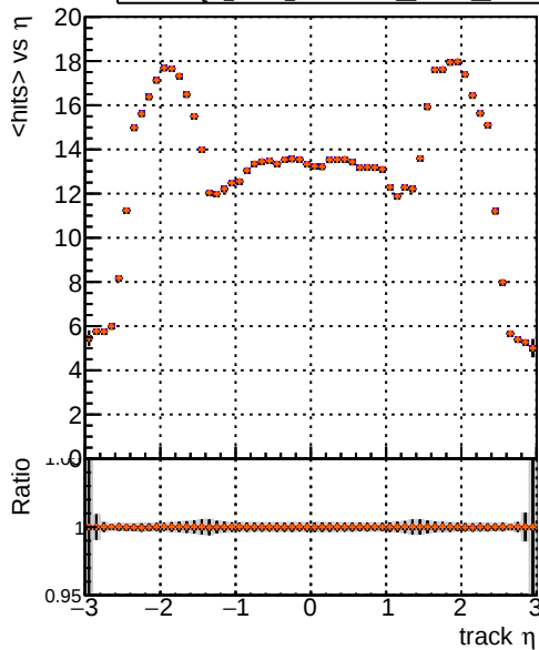
mean hit DQM_V0001_R0000000001_Global_CMSSW_orig DQM_V0001_R0000000001_Global_CMSSW_pl08 DQM_V0001_R0000000001_Global_CMSSW_pl075 DQM_V0001_R0000000001_Global_CMSSW_pl07
