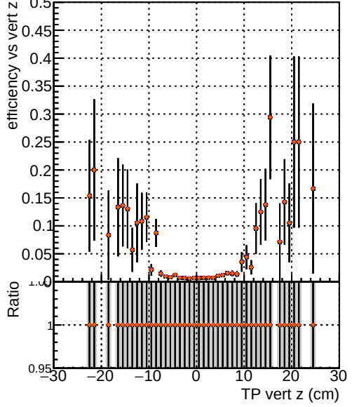
Efficiency vs vert z —●— DQM_V0001_R000000001 Global CMSSW_orig —●— DQM_V0001_R000000001 Global CMSSW_pl08 —●— DQM_V0001_R000000001 Global CMSSW_pl075 —●— DQM_V0001_R000000001 Global CMSSW_pl07
