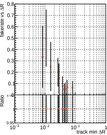
Fake rate vs ΔR(track, jet) | DQM V00001 R00000000001 Global CMSSW orig DQM V00001 R00000000001 Global CMSSW pb075 DQM V00001 R00000000001 Global CMSSW pb075
