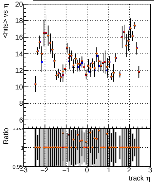
mean hits Legend: DQM_V0001_R000000001_Global_CMSSW_orig, DQM_V0001_R000000001_Global_CMSSW_pl08, DQM_V0001_R000000001_Global_CMSSW_pl075, DQM_V0001_R000000001_Global_CMSSW_pl07
