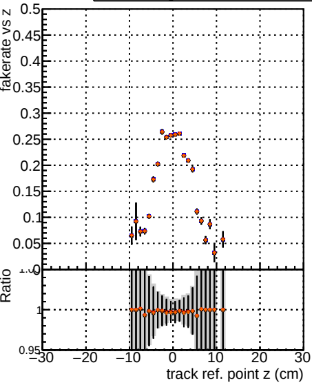
Fake rate vs v DOM V0001 R0000000001 Global DOM V0001 R0000000001 Global DOM V0001 R0000000001 Global CMSSW orig CMSSW p075
