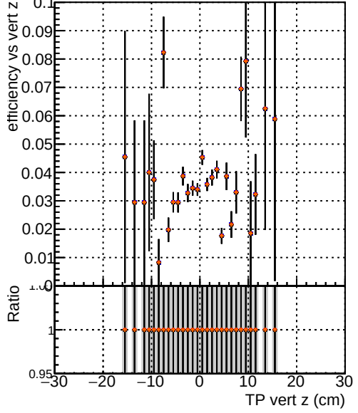
Efficiency vs. sim PV z —●— DQM_V0001_R000000001 Global CMSSW_orig —●— DQM_V0001_R000000001 Global CMSSW_pl08 —●— DQM_V0001_R000000001 Global CMSSW_pl075 —●— DQM_V0001_R000000001 Global CMSSW_pl07
