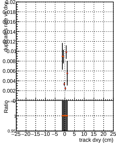
Legend for Fake rate vs dxy, Duplicates Rate vs Dxy, and Pileup rate vs dxy: Global CMSSW_8_0_0 CMSSW_8_0_1 CMSSW_8_0_2 CMSSW_8_0_3 CMSSW_8_0_4 CMSSW_8_0_5 CMSSW_8_0_6 CMSSW_8_0_7 CMSSW_8_0_8 CMSSW_8_0_9 CMSSW_8_1_0 CMSSW_8_1_1 CMSSW_8_1_2 CMSSW_8_1_3 CMSSW_8_1_4 CMSSW_8_1_5 CMSSW_8_1_6 CMSSW_8_1_7 CMSSW_8_1_8 CMSSW_8_1_9 CMSSW_8_2_0 CMSSW_8_2_1 CMSSW_8_2_2 CMSSW_8_2_3 CMSSW_8_2_4 CMSSW_8_2_5 CMSSW_8_2_6 CMSSW_8_2_7 CMSSW_8_2_8 CMSSW_8_2_9 CMSSW_8_3_0 CMSSW_8_3_1 CMSSW_8_3_2 CMSSW_8_3_3 CMSSW_8_3_4 CMSSW_8_3_5 CMSSW_8_3_6 CMSSW_8_3_7 CMSSW_8_3_8 CMSSW_8_3_9 CMSSW_8_4_0 CMSSW_8_4_1 CMSSW_8_4_2 CMSSW_8_4_3 CMSSW_8_4_4 CMSSW_8_4_5 CMSSW_8_4_6 CMSSW_8_4_7 CMSSW_8_4_8 CMSSW_8_4_9 CMSSW_8_5_0 CMSSW_8_5_1 CMSSW_8_5_2 CMSSW_8_5_3 CMSSW_8_5_4 CMSSW_8_5_5 CMSSW_8_5_6 CMSSW_8_5_7 CMSSW_8_5_8 CMSSW_8_5_9 CMSSW_8_6_0 CMSSW_8_6_1 CMSSW_8_6_2 CMSSW_8_6_3 CMSSW_8_6_4 CMSSW_8_6_5 CMSSW_8_6_6 CMSSW_8_6_7 CMSSW_8_6_8 CMSSW_8_6_9 CMSSW_8_7_0 CMSSW_8_7_1 CMSSW_8_7_2 CMSSW_8_7_3 CMSSW_8_7_4 CMSSW_8_7_5 CMSSW_8_7_6 CMSSW_8_7_7 CMSSW_8_7_8 CMSSW_8_7_9 CMSSW_8_8_0 CMSSW_8_8_1 CMSSW_8_8_2 CMSSW_8_8_3 CMSSW_8_8_4 CMSSW_8_8_5 CMSSW_8_8_6 CMSSW_8_8_7 CMSSW_8_8_8 CMSSW_8_8_9 CMSSW_8_9_0 CMSSW_8_9_1 CMSSW_8_9_2 CMSSW_8_9_3 CMSSW_8_9_4 CMSSW_8_9_5 CMSSW_8_9_6 CMSSW_8_9_7 CMSSW_8_9_8 CMSSW_8_9_9 CMSSW_9_0_0 CMSSW_9_0_1 CMSSW_9_0_2 CMSSW_9_0_3 CMSSW_9_0_4 CMSSW_9_0_5 CMSSW_9_0_6 CMSSW_9_0_7 CMSSW_9_0_8 CMSSW_9_0_9 CMSSW_9_1_0 CMSSW_9_1_1 CMSSW_9_1_2 CMSSW_9_1_3 CMSSW_9_1_4 CMSSW_9_1_5 CMSSW_9_1_6 CMSSW_9_1_7 CMSSW_9_1_8 CMSSW_9_1_9 CMSSW_9_2_0 CMSSW_9_2_1 CMSSW_9_2_2 CMSSW_9_2_3 CMSSW_9_2_4 CMSSW_9_2_5 CMSSW_9_2_6 CMSSW_9_2_7 CMSSW_9_2_8 CMSSW_9_2_9 CMSSW_9_3_0 CMSSW_9_3_1 CMSSW_9_3_2 CMSSW_9_3_3 CMSSW_9_3_4 CMSSW_9_3_5 CMSSW_9_3_6 CMSSW_9_3_7 CMSSW_9_3_8 CMSSW_9_3_9 CMSSW_9_4_0 CMSSW_9_4_1 CMSSW_9_4_2 CMSSW_9_4_3 CMSSW_9_4_4 CMSSW_9_4_5 CMSSW_9_4_6 CMSSW_9_4_7 CMSSW_9_4_8 CMSSW_9_4_9 CMSSW_9_5_0 CMSSW_9_5_1 CMSSW_9_5_2 CMSSW_9_5_3 CMSSW_9_5_4 CMSSW_9_5_5 CMSSW_9_5_6 CMSSW_9_5_7 CMSSW_9_5_8 CMSSW_9_5_9 CMSSW_9_6_0 CMSSW_9_6_1 CMSSW_9_6_2 CMSSW_9_6_3 CMSSW_9_6_4 CMSSW_9_6_5 CMSSW_9_6_6 CMSSW_9_6_7 CMSSW_9_6_8 CMSSW_9_6_9 CMSSW_9_7_0 CMSSW_9_7_1 CMSSW_9_7_2 CMSSW_9_7_3 CMSSW_9_7_4 CMSSW_9_7_5 CMSSW_9_7_6 CMSSW_9_7_7 CMSSW_9_7_8 CMSSW_9_7_9 CMSSW_9_8_0 CMSSW_9_8_1 CMSSW_9_8_2 CMSSW_9_8_3 CMSSW_9_8_4 CMSSW_9_8_5 CMSSW_9_8_6 CMSSW_9_8_7 CMSSW_9_8_8 CMSSW_9_8_9 CMSSW_9_9_0 CMSSW_9_9_1 CMSSW_9_9_2 CMSSW_9_9_3 CMSSW_9_9_4 CMSSW_9_9_5 CMSSW_9_9_6 CMSSW_9_9_7 CMSSW_9_9_8 CMSSW_9_9_9
