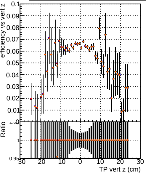
—●— DQM_V0001_R0000000001 Global CMSSW_orig —●— DQM_V0001_R0000000001 Global CMSSW_pl08 —●— DQM_V0001_R0000000001 Global CMSSW_pl075 —●— DQM_V0001_R0000000001 Global CMSSW_pl07
