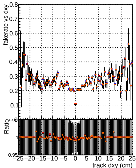
Legend for Fake rate vs dxy: Global CMSSW 8.0.0 CMSSW 8.0.1 CMSSW 8.0.2 CMSSW 8.0.3 CMSSW 8.0.4 CMSSW 8.0.5 CMSSW 8.0.6 CMSSW 8.0.7 CMSSW 8.0.8 CMSSW 8.0.9 CMSSW 8.1.0 CMSSW 8.1.1 CMSSW 8.1.2 CMSSW 8.1.3 CMSSW 8.1.4 CMSSW 8.1.5 CMSSW 8.1.6 CMSSW 8.1.7 CMSSW 8.1.8 CMSSW 8.1.9 CMSSW 8.2.0 CMSSW 8.2.1 CMSSW 8.2.2 CMSSW 8.2.3 CMSSW 8.2.4 CMSSW 8.2.5 CMSSW 8.2.6 CMSSW 8.2.7 CMSSW 8.2.8 CMSSW 8.2.9 CMSSW 8.3.0 CMSSW 8.3.1 CMSSW 8.3.2 CMSSW 8.3.3 CMSSW 8.3.4 CMSSW 8.3.5 CMSSW 8.3.6 CMSSW 8.3.7 CMSSW 8.3.8 CMSSW 8.3.9 CMSSW 8.4.0 CMSSW 8.4.1 CMSSW 8.4.2 CMSSW 8.4.3 CMSSW 8.4.4 CMSSW 8.4.5 CMSSW 8.4.6 CMSSW 8.4.7 CMSSW 8.4.8 CMSSW 8.4.9 CMSSW 8.5.0 CMSSW 8.5.1 CMSSW 8.5.2 CMSSW 8.5.3 CMSSW 8.5.4 CMSSW 8.5.5 CMSSW 8.5.6 CMSSW 8.5.7 CMSSW 8.5.8 CMSSW 8.5.9 CMSSW 8.6.0 CMSSW 8.6.1 CMSSW 8.6.2 CMSSW 8.6.3 CMSSW 8.6.4 CMSSW 8.6.5 CMSSW 8.6.6 CMSSW 8.6.7 CMSSW 8.6.8 CMSSW 8.6.9 CMSSW 8.7.0 CMSSW 8.7.1 CMSSW 8.7.2 CMSSW 8.7.3 CMSSW 8.7.4 CMSSW 8.7.5 CMSSW 8.7.6 CMSSW 8.7.7 CMSSW 8.7.8 CMSSW 8.7.9 CMSSW 8.8.0 CMSSW 8.8.1 CMSSW 8.8.2 CMSSW 8.8.3 CMSSW 8.8.4 CMSSW 8.8.5 CMSSW 8.8.6 CMSSW 8.8.7 CMSSW 8.8.8 CMSSW 8.8.9 CMSSW 8.9.0 CMSSW 8.9.1 CMSSW 8.9.2 CMSSW 8.9.3 CMSSW 8.9.4 CMSSW 8.9.5 CMSSW 8.9.6 CMSSW 8.9.7 CMSSW 8.9.8 CMSSW 8.9.9 CMSSW 9.0.0 CMSSW 9.0.1 CMSSW 9.0.2 CMSSW 9.0.3 CMSSW 9.0.4 CMSSW 9.0.5 CMSSW 9.0.6 CMSSW 9.0.7 CMSSW 9.0.8 CMSSW 9.0.9 CMSSW 9.1.0 CMSSW 9.1.1 CMSSW 9.1.2 CMSSW 9.1.3 CMSSW 9.1.4 CMSSW 9.1.5 CMSSW 9.1.6 CMSSW 9.1.7 CMSSW 9.1.8 CMSSW 9.1.9 CMSSW 9.2.0 CMSSW 9.2.1 CMSSW 9.2.2 CMSSW 9.2.3 CMSSW 9.2.4 CMSSW 9.2.5 CMSSW 9.2.6 CMSSW 9.2.7 CMSSW 9.2.8 CMSSW 9.2.9 CMSSW 9.3.0 CMSSW 9.3.1 CMSSW 9.3.2 CMSSW 9.3.3 CMSSW 9.3.4 CMSSW 9.3.5 CMSSW 9.3.6 CMSSW 9.3.7 CMSSW 9.3.8 CMSSW 9.3.9 CMSSW 9.4.0 CMSSW 9.4.1 CMSSW 9.4.2 CMSSW 9.4.3 CMSSW 9.4.4 CMSSW 9.4.5 CMSSW 9.4.6 CMSSW 9.4.7 CMSSW 9.4.8 CMSSW 9.4.9 CMSSW 9.5.0 CMSSW 9.5.1 CMSSW 9.5.2 CMSSW 9.5.3 CMSSW 9.5.4 CMSSW 9.5.5 CMSSW 9.5.6 CMSSW 9.5.7 CMSSW 9.5.8 CMSSW 9.5.9 CMSSW 9.6.0 CMSSW 9.6.1 CMSSW 9.6.2 CMSSW 9.6.3 CMSSW 9.6.4 CMSSW 9.6.5 CMSSW 9.6.6 CMSSW 9.6.7 CMSSW 9.6.8 CMSSW 9.6.9 CMSSW 9.7.0 CMSSW 9.7.1 CMSSW 9.7.2 CMSSW 9.7.3 CMSSW 9.7.4 CMSSW 9.7.5 CMSSW 9.7.6 CMSSW 9.7.7 CMSSW 9.7.8 CMSSW 9.7.9 CMSSW 9.8.0 CMSSW 9.8.1 CMSSW 9.8.2 CMSSW 9.8.3 CMSSW 9.8.4 CMSSW 9.8.5 CMSSW 9.8.6 CMSSW 9.8.7 CMSSW 9.8.8 CMSSW 9.8.9 CMSSW 9.9.0 CMSSW 9.9.1 CMSSW 9.9.2 CMSSW 9.9.3 CMSSW 9.9.4 CMSSW 9.9.5 CMSSW 9.9.6 CMSSW 9.9.7 CMSSW 9.9.8 CMSSW 9.9.9
